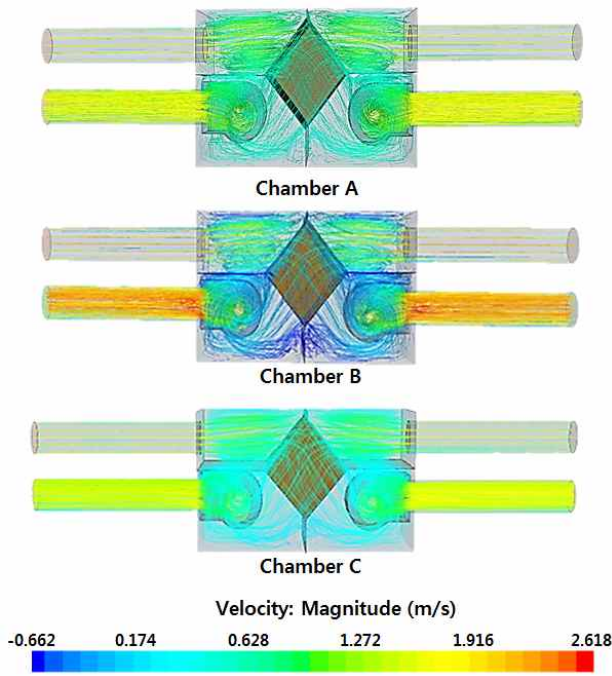
Fig. 7 Airflow distribution of chamber.
