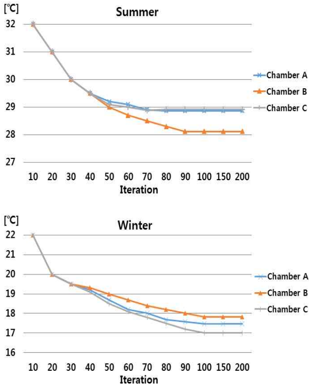
Fig. 8 Temperature distribution of supply air duct.
