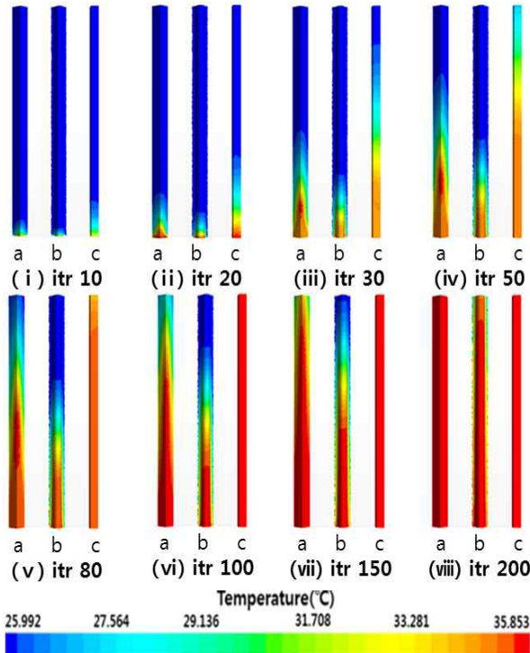
Fig. 6 Heat transfer distribution of element.
