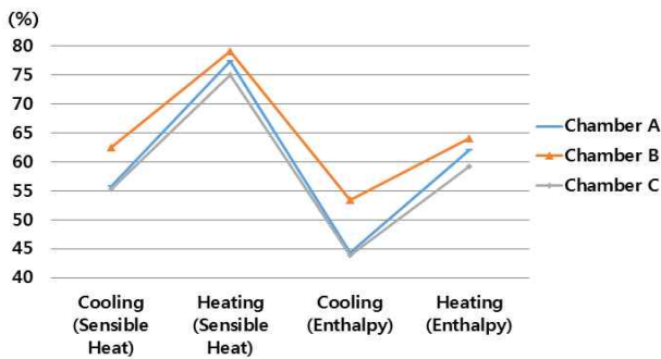
Fig. 9 Efficiencies of heat and enthalpy exchangers.
