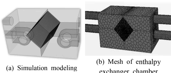
Fig. 5 Simulation model and mesh of STAR-CCM+
