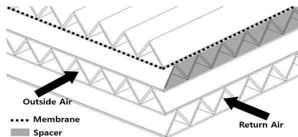
Fig. 2 Schematic drawing of the enthalpy exchanger.
