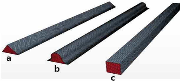
Fig. 3 Grid generation of enthalpy exchanger elements.
